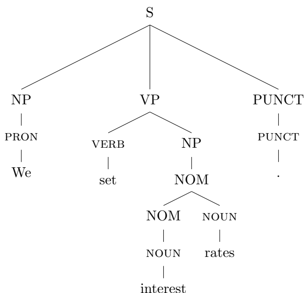
Fig. 12. Syntactic constituency parse for an example sentence: “We set interest rates.”
